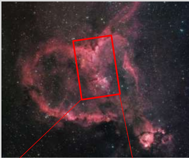
APOD 2009 February 14 IC 1805: The Heart Nebula Credit & Copyright: Daniel Marquardt
