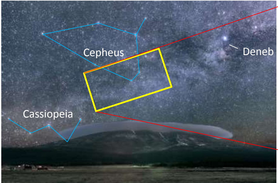
2008 April 16 A Protected Night Sky Over Flagstaff Credit and Copyright: Dan & Cindy Duriscoe, FDSC, Lowell Obs., USNO
